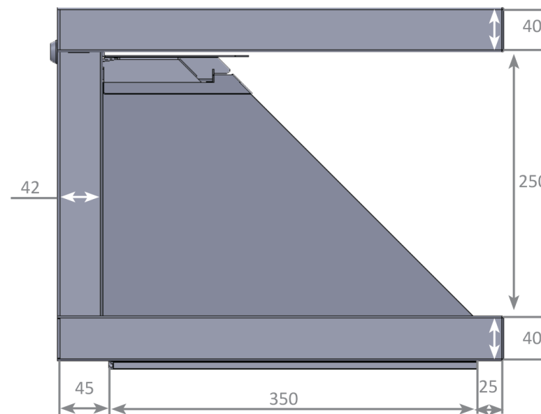
Dreamoc HD3 left side - measurements
