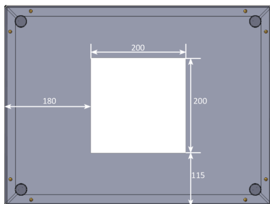
Dreamoc HD3 Stand bottom - measurements
